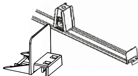
Frontanker gerade 40x35 mm
